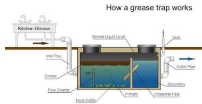
EXTERNAL TRAPS https://i.pinimg.com/originals/a4/81/b1/a481b1d870953f150cb0bc8a8b24881f.jpg
